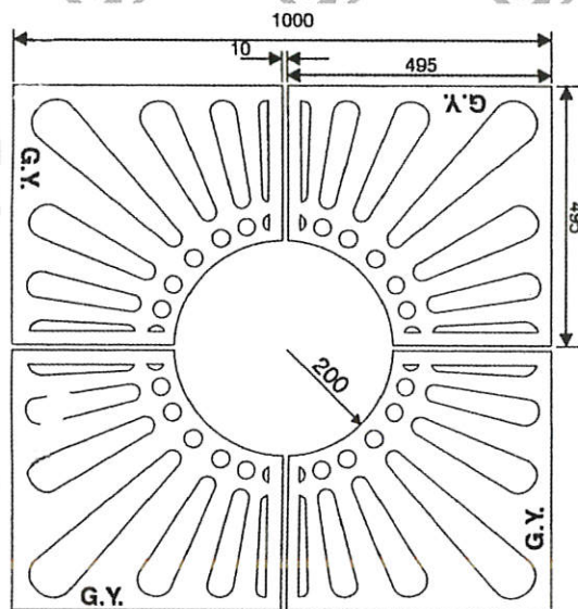
“G.Y.” 1000x1000x40厚太陽花種樹梳冷
