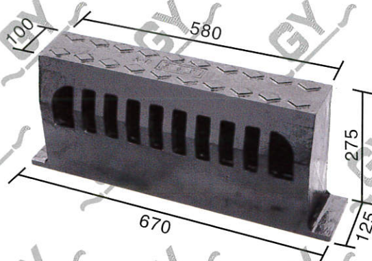
G.Y. 牌馬路邊梳冷篋仔 G.Y. Brand Kerb Overflow Weir Type K1-450V
