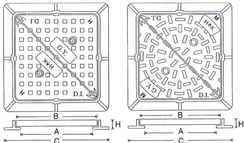
“G.Y.” 牌球鐵雙三角沙井蓋板 “G.Y.” Brand D.I. Double Triangular Manhole Cover & Frame
