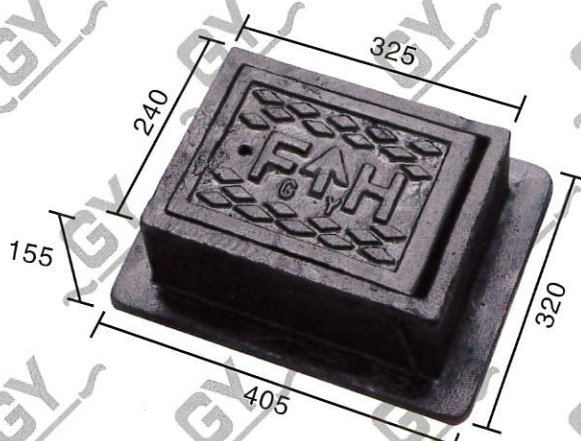
G.Y. 牌消防正 G.Y. Brand C.I. Fire Hydrant Cover
