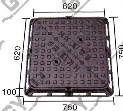
“G.Y.” 牌球鐵雙三角梳冷蓋板 “G.Y.” Brand D.I. Double Triangular Gully Grating
