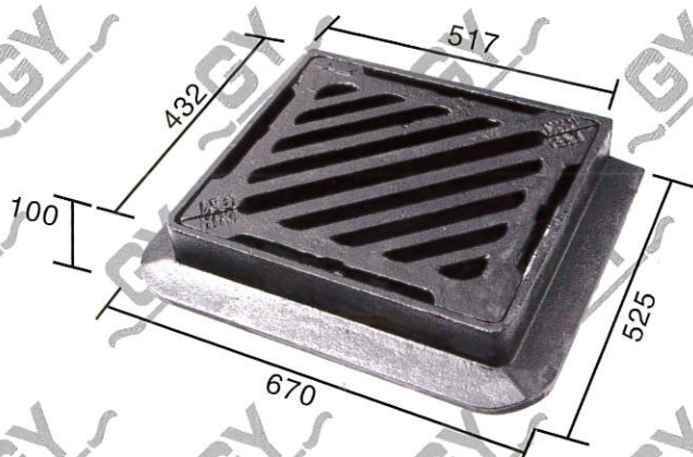
G.Y. 牌有框雙三角梳冷 (三邊) G.Y. Brand Double Triangular Gully Grating Type GA1-450
