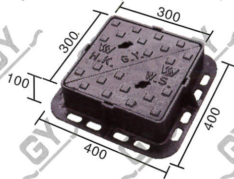
“G.Y.” 牌球鐵消防蓋 “G.Y.” Brand D.I. Fire Hydrant Cover
