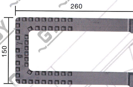
G.Y. 牌腳踏/ G.Y. Brand Step Iron
