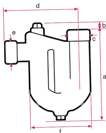
"G.Y." Brand BS416 50mm Anti-Syphon "P" Trap "G.Y."牌 BS416 2"防啞力格氣
