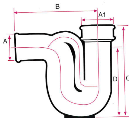
"G.Y." Brand BS416 Anti-syphon "P" Trap With Door "G.Y."牌 BS416 有口"P"型防啞力格氣
