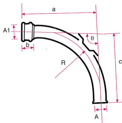
"G.Y." Brand BS416 Running Trap With Door "G.Y."牌 BS416 有口牛押曲
