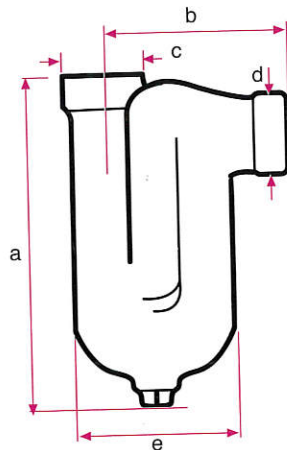
"G.Y." Brand BS416 40mm Anti-Syphon "P" Trap "G.Y."牌 BS416 1.5"防啞力格氣
